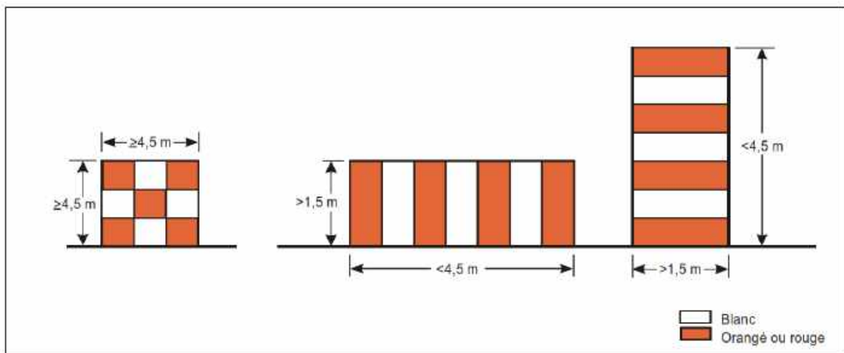
Figure 6-1. Marquages types
